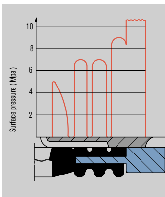
Distribution of contact forces with an EagleBurgmann 9107/KN gasket in a non-load bearing, rubberized flange connection.
