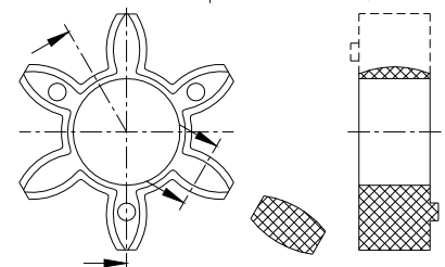
Illustration 17.2: ROTEX® spider
