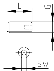
Illustration 13: Withworth setscrew (BSW)
