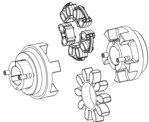
Type with taper clamping sleeve
