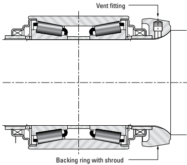
Fig. 36 Mounting Arrangement 2
