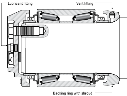
Fig. 34 Mounting Arrangement 1
