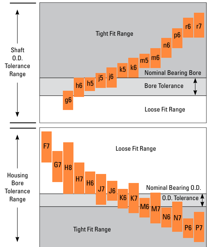
Fig. 2. Shaft and housing fit selection.
